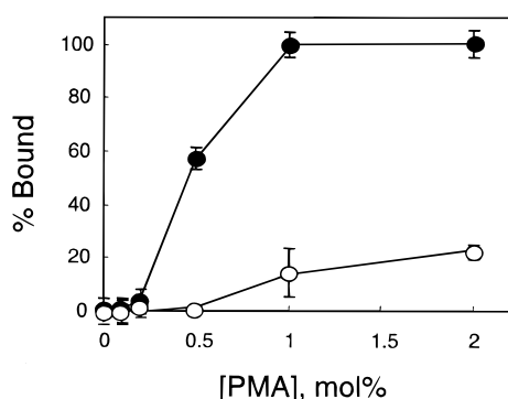
FIGURE 2: PMA recruits the C1B domain to neutral and anionic membranes. Binding of the C1B domain to phosphatidylcholine (open symbols) or phosphatidylserine/phosphatidylcholine vesicles (40:60 mole fraction; solid symbols) containing 0–2 mol % PMA was measured as described under Materials and Methods. Total lipid concentration was 1 mM. Membrane binding was measured in the presence of 100 mM KCl and 2.5 mM MgCl 2 . Data represent the average \pm range of duplicate determinations from a representative experiment.
