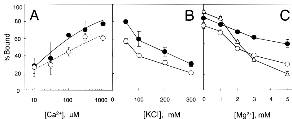
FIGURE 9: Dependence of the C2 domain/membrane interaction on calcium, ionic strength, and magnesium. The binding of the C2 domain to phosphatidylcholine vesicles containing 40 mol % phosphatidylglycerol (open circles), phosphatidylserine (closed circles), or phosphatidic acid (open triangles) was measured in the presence of various ion concentrations as described under Materials and Methods. The total lipid concentration was 0.5 mM. Unless otherwise indicated, ion concentrations were 100 mM KCl, 5 mM MgCl 2 , and 0.3 mM calcium. Data represent the average \pm range of duplicate determinations from representative experiments. (A) The binding of the C2 domain to membranes was measured in the presence of 10–1000 \mu M free Ca 2+ using 0.5 mM EGTA as a buffer, as described (44). (B) The binding of the C2 domain to membranes was measured in the presence of 50–300 mM KCl. (C) The binding of the C2 domain to membranes was measured in the presence of 0–5 mM MgCl 2 .
