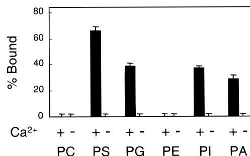
FIGURE 7: Lipid selectivity in the interaction of the C2 domain with membranes. The binding of the C2 domain to phosphatidylcholine vesicles (PC) or phosphatidylcholine vesicles containing 40 mol % phosphatidylserine (PS), phosphatidylglycerol (PG), phosphatidylethanolamine (PE), phosphatidylinositol (PI), or phosphatidic acid (PA) was measured in the presence of 0.3 mM calcium (solid bars) or 0.5 mM EGTA (open bars) as described under Materials and Methods. The total lipid concentration was 0.5 mM. Membrane binding was measured in the presence of 100 mM KCl and 5 mM \text{MgCl}_2 . Data represent the average \pm SEM of 6 determinations.
