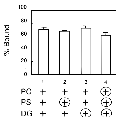
FIGURE 8: Interaction of the C2 domain with phosphatidylserine is not stereospecific. The binding of the C2 domain to diacylglycerol/phosphatidylserine/phosphatidylcholine (5:40:55, mole fraction) vesicles containing various stereoisomers was measured as described under Materials and Methods. (1) Vesicles contained natural isomers ( sn -1,2-phosphatidyl-L-serine, sn -1,2-diacylglycerol, sn -1,2-phosphatidylcholine); (2) the phosphatidylserine enantiomer ( sn -2,3-phosphatidyl-D-serine, sn -1,2-diacylglycerol, sn -1,2-phosphatidylcholine); (3) the diacylglycerol enantiomer ( sn -1,2-phosphatidyl-L-serine, sn -2,3-diacylglycerol, sn -1,2-phosphatidylcholine); or (4) enantiomers of all three components ( sn -2,3-phosphatidyl-D-serine, sn -2,3-diacylglycerol, sn -2,3-phosphatidylcholine). The total lipid concentration was 0.5 mM. Membrane binding was measured in the presence of 0.3 mM \text{Ca}^{2+} , 100 mM KCl, and 5 mM \text{MgCl}_2 . Data represent the average \pm SEM of 6 determinations. Circled lipids indicate the sn -2,3 stereochemistry.
