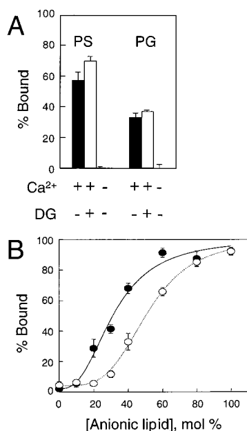
FIGURE 6: Binding of the C2 domain to membranes is dependent on anionic lipid and \text{Ca}^{2+} . (A) The binding of the C2 domain to phosphatidylcholine vesicles containing 40 mol % phosphatidylserine (PS) or phosphatidylglycerol (PG) was measured in the absence (solid bars) or presence (open bars) of 5 mol % diacylglycerol (DG) and in the presence of 0.3 mM \text{Ca}^{2+} (open and solid bars) or 0.5 mM EGTA, as described under Materials and Methods. The total lipid concentration was 0.5 mM. Membrane binding was measured in the presence of 100 mM KCl and 5 mM \text{MgCl}_2 . Data are average \pm range of duplicate determinations from a representative experiment. (B) The binding of the C2 domain to phosphatidylcholine vesicles containing the indicated amount of phosphatidylglycerol (open symbols) or phosphatidylserine (solid symbols) was measured as described under Materials and Methods. The total lipid concentration was 0.5 mM. Assays contained 0.3 mM \text{Ca}^{2+} , 100 mM KCl, and 5 mM \text{MgCl}_2 . Data represent the average \pm SEM of 4–6 determinations. The curves shown are predicted for the data from a modified Hill equation using Sigma plot, as described previously (43).
