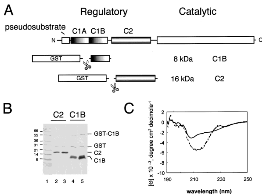
FIGURE 1: C1B and C2 domain constructs. (A) Schematic representation of C1B domain (residues 92–161 of protein kinase C \beta II) and C2 domain (residues 157–289) constructs used in this study. Proteins were expressed as fusion proteins with GST, which was subsequently removed as described under Materials and Methods. (B) Coomassie-stained gel of the purified C2 (lanes 2 and 3, 1.3 and 3.3 \mu g) and C1B domains (lanes 4 and 5, 3 and 7.5 \mu g). (C) Circular dichroism spectra of the purified C2 (dashed line) and C1B (solid line) domains, measured as described under Materials and Methods. Protein concentrations were 0.65 and 1.5 mg mL -1 for the C2 and C1B domains, respectively.
