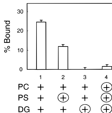
FIGURE 5: Binding of the C1B domain to phosphatidylserine is stereospecific. The binding of the C1B domain to diacylglycerol/phosphatidylserine/phosphatidylcholine (5:40:55 mole fraction) vesicles containing various stereoisomers was measured as described under Materials and Methods. (1) Vesicles contained natural isomers ( sn -1,2-phosphatidyl-L-serine, sn -1,2-diacylglycerol, sn -1,2-phosphatidylcholine); (2) the phosphatidylserine enantiomer ( sn -2,3-phosphatidyl-D-serine, sn -1,2-diacylglycerol, sn -1,2-phosphatidylcholine); (3) the diacylglycerol enantiomer ( sn -1,2-phosphatidyl-L-serine, sn -2,3-diacylglycerol, sn -1,2-phosphatidylcholine); or (4) enantiomers of all three components ( sn -2,3-phosphatidyl-D-serine, sn -2,3-diacylglycerol, sn -2,3-phosphatidylcholine). The total lipid concentration was 1 mM. Membrane binding was measured in the presence of 100 mM KCl and 2.5 mM \text{MgCl}_2 . Data represent the average \pm SEM of 6 determinations. Circled lipids indicate the sn -2,3 stereochemistry.
