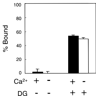
FIGURE 3: Diacylglycerol, but not \text{Ca}^{2+} , modulates the affinity of the C1B domain for anionic membranes. Binding of the C1B domain to phosphatidylcholine vesicles containing phosphatidylserine (40 mol %), with or without 5 mol % diacylglycerol (DG), was measured in the presence of 0.3 mM \text{Ca}^{2+} (solid bars) or 0.5 mM EGTA (open bars) as described under Materials and Methods. Total lipid concentration was 1 mM. Membrane binding was measured in the presence of 100 mM KCl and 2.5 mM \text{MgCl}_2 . Data represent the average \pm range of duplicate determinations from a representative experiment.
