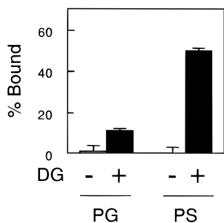
FIGURE 4: C1B domain selectively binds phosphatidylserine-containing membranes. (A) The binding of the C1B domain to phosphatidylcholine vesicles containing 40 mol % phosphatidylglycerol (PG) (left) or 40 mol % phosphatidylserine (PS) (right) was measured in the presence or absence of 5 mol % diacylglycerol (DG) as described under Materials and Methods. Total lipid concentration was 1 mM. Binding measurements were conducted in the presence of 100 mM KCl and 2.5 mM \text{MgCl}_2 . Data represent the average \pm SEM of 4–6 determinations.
